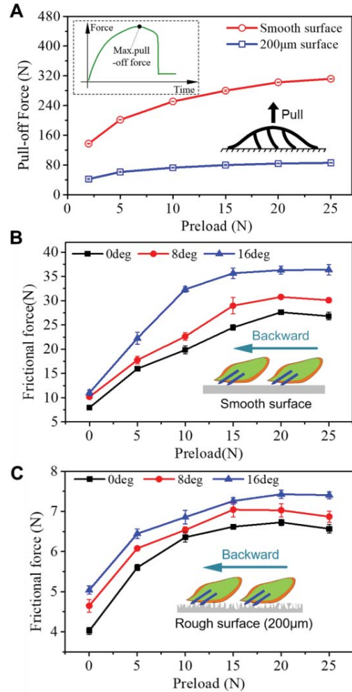
Fig. 4. The adhesive performance of the biomimetic remora disc. (A) The maximum pull-off force of the biomimetic disc prototype for different preloads on a smooth surface (surface roughness R_a = 0 \mu\text{m} ) and a rough surface ( R_a = 200 \mu\text{m} ). (Inset) Vertically directed pull-off force time series (smooth surface, preload 10 N) and location of maximum pull-off force. Backward frictional force of the disc prototype at 0^\circ , 8^\circ , and 16^\circ lamellae pitch angles under variable preloads on a (B) smooth surface and (C) rough surface ( R_a = 200 \mu\text{m} ). 5 replicate trials were performed for each experimental scenario. Error bars indicate the standard deviations.
