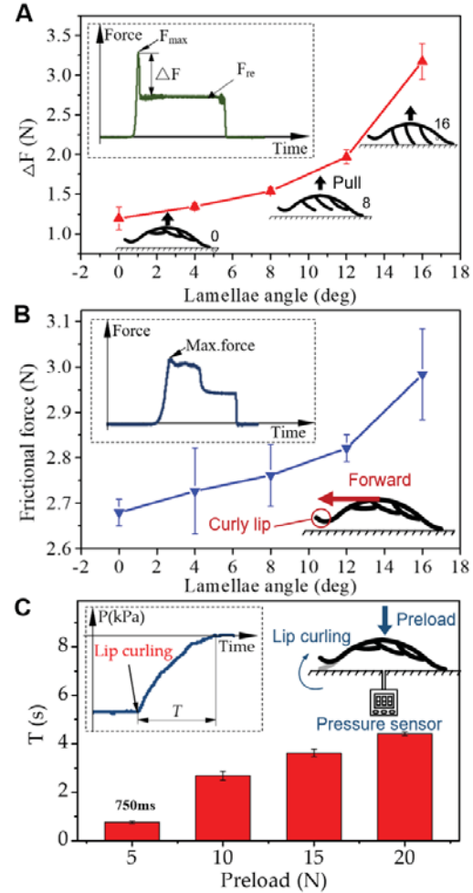
Fig. 5. Performance of the biomimetic remora disc prototype during detachment (underwater, soft lip in curling state, smooth surface). (A) Surface adhesion \Delta F ( F_{max}-F_{re} , with the soft lip curling up) increased with the lamellae pitch angles ( \theta = 0^\circ, 4^\circ, 8^\circ, 12^\circ, 16^\circ ). Inset panel: vertically directed pull-off force as a function of time (underwater, soft lip in curling state, smooth surface), maximum pull-off force ( F_{max} ), and average remaining weight ( F_{re} ). (B) Maximum forward frictional force increased with the lamellae pitch angles ( \theta = 0^\circ, 4^\circ, 8^\circ, 12^\circ, 16^\circ ). (Inset) Frictional force ( \theta = 8^\circ ) as a function of time. (C) Detachment time of the disc prototype under different preloads (smooth surface, underwater). Detachment time ( T ) represents the period from the start of the lip curl to full detachment. Inset panels indicate the change in inner-chamber pressure of the disc as a function of time. The pressure sensor was located at the center of the disc. 5 replicate trials were performed for each experimental scenario. Error bars indicate the standard deviations.
