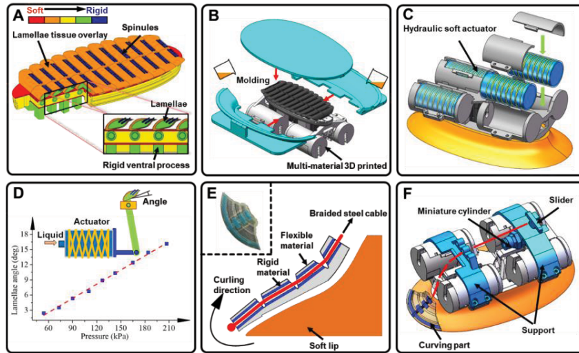
Fig. 2. Design and fabrication of the biomimetic remora disc prototype. (A) CAD model of the main disc and the lamellae mechanisms. Different colors correspond to different stiffness (from 10^4 \sim 10^{11} Pa). DPSS laser machined artificial spinules (blue) are the most rigid part of the disc (Young's Modulus: \sim 2 \times 10^{11} Pa). The main disc structure was printed with a multi-material 3D printer (Objet Connex500 C3). (B) The silicone elastomeric soft lip was fabricated and bonded to the lamellae mechanism through multi-step mold and cast approach. (C) Hydraulic soft actuators for actuating the disc lamellae. (D) The lamellae pitch angle ( \theta ) increases linearly as a function of hydraulic pressure. (E) Cross-sectional schematic of the detachment mechanism. The internal channels (blue) and covering layer (translucent) were simultaneously printed with rigid and flexible materials, respectively. (F) Disc detachment is realized by the cable-driven curling mechanism that includes the 3D-printed curling section, the miniature hydraulic cylinder, and the slider mechanism. The pulling force for detachment is exerted from the pressure in the miniature hydraulic cylinder.
