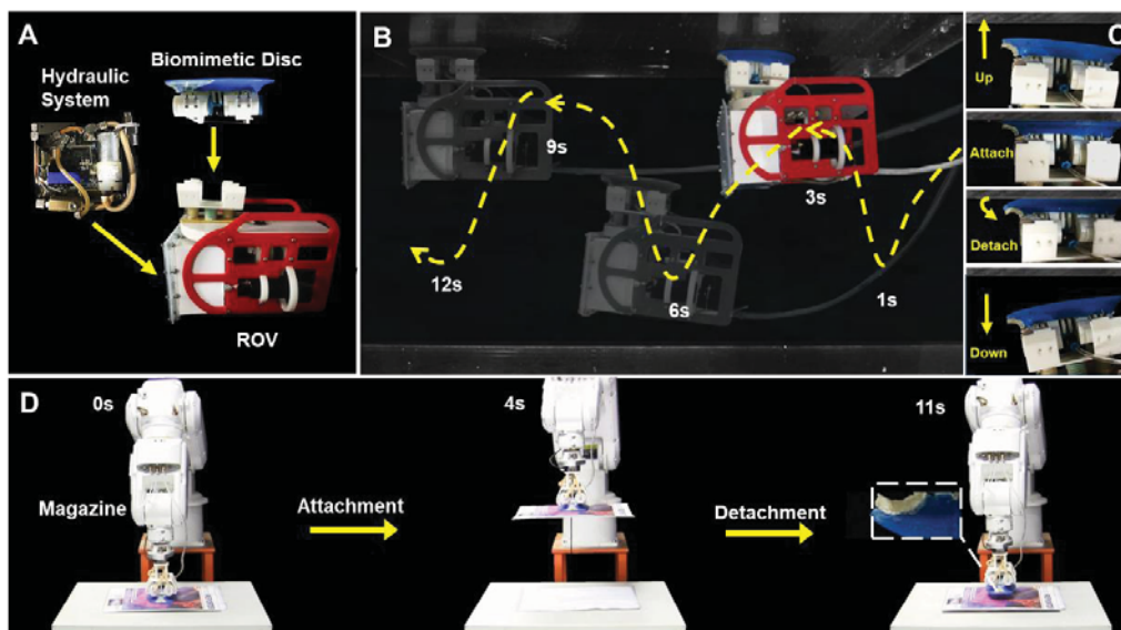
Fig. 6. Verification tests of the attachment and detachment performance of the biomimetic remora disc. (A) An integrated underwater vehicle. The biomimetic remora disc was mounted on the ROV through a connection device that included four springs and four soft silicone hydraulic elastomer actuators. A hydraulic system was connected to the front of the ROV to control the disc's curling mechanism and lamellae motion. (B) The integrated ROV can switch seamlessly between attachment and detachment. (B) shows two continuous attachment and detachment maneuvers on a smooth surface within 12 s. Scale bar 5 cm. (C) A complete attachment and detachment maneuver that shows the details of the disc's motion. Scale bar 3 cm. (D) Demonstration of gripping and releasing a magazine in air. Scale bar 10 cm.
