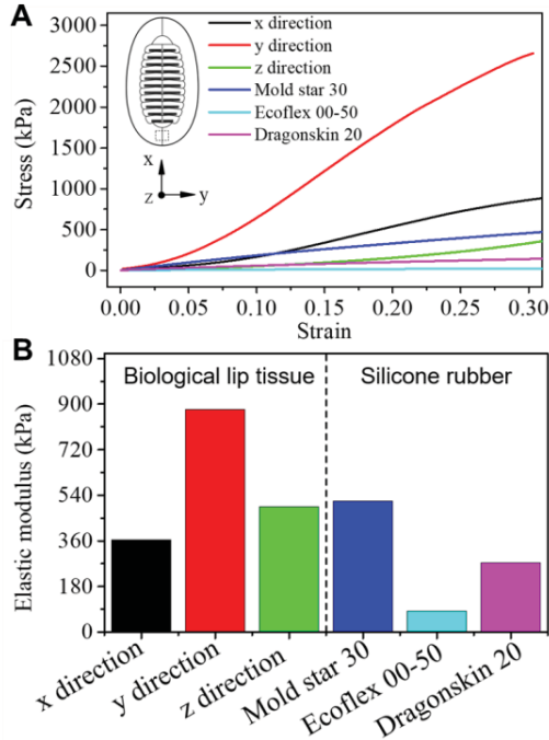
Fig. 3. The mechanical properties of the biological and biomimetic soft lip. (A) Stress-strain curves of fresh remora lip tissue (x, y, and z directions) and several silicone elastomeric materials (Mold star 30, Ecoflex 00-50, Dragonskin 20, Smooth-On Inc., PA, USA). (Inset) Schematic of remora disc with the position of fleshy lip sample and x, y, and z axes indicated. (B) Elastic modulus (gradient of stress-strain curves) of the fleshy lip and the silicone elastomeric materials.
